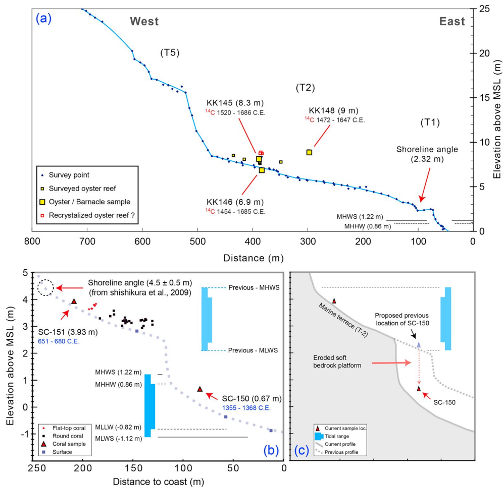
Figure 13. (a) A topographic profile north of the village of Kan-Daing-Ok (the location of the profile is shown in Figure 12). Here uplifted shoreline angle and oyster reefs show \sim 1.1 m of land-level change after the 17th century. The 15th to 16th century radiocarbon ages of the oysters on T2 suggest that the lowest terrace (T1) formed after the 17th century, likely during the 1762 earthquake. (b) The shoreline angle of T2 and the U-Th age of an eroded coral (SC-150) near the modern high tide suggest 1.5 to \sim 3 m of land-level change after the 14th century south of Kan-Daing-Ok. The topography profile and the elevation of the shoreline angle are modified after Shishikura et al. [2009]. The location of this profile is shown in Figure 12. (c) A proposed differential erosion model to interpret the elevation of sample SC-150. See text for discussion.
