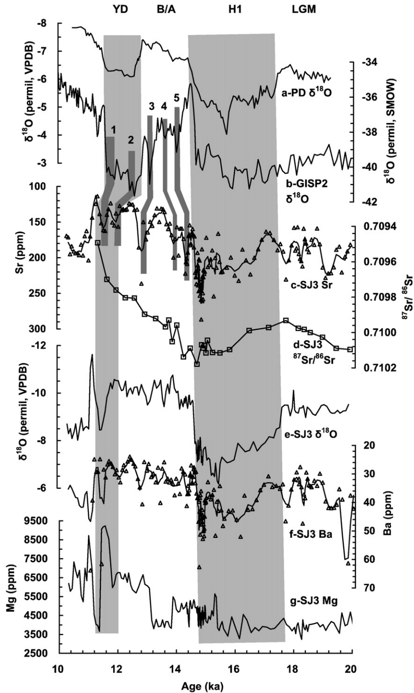
Fig. 8. Comparison of the Sr concentration (c) and 87 Sr/ 86 Sr ratio (d) variations of SJ3 with the speleothem δ 18 O records of the same stalagmite (SJ3) (Zhou et al., 2008a) (e) and PD from Hulu cave in East China (Wang et al., 2001) (a), and the polar ice core δ 18 O record (Grootes et al., 1993; Stuiver et al., 1995) (b). Also shown are the Ba (f) and Mg (g) records of SJ3. The solid line in (c), (f) and (g) represents a three-point running average trend of the data. The longer light grey bars indicate the two cold phases of the Younger Dryas and H1 events. The five shorter grey bars marked with 1–5 indicate small Sr peaks corresponding to five centennial cold events in the polar ice core during the B/A warm period and the YD cold reversal.
