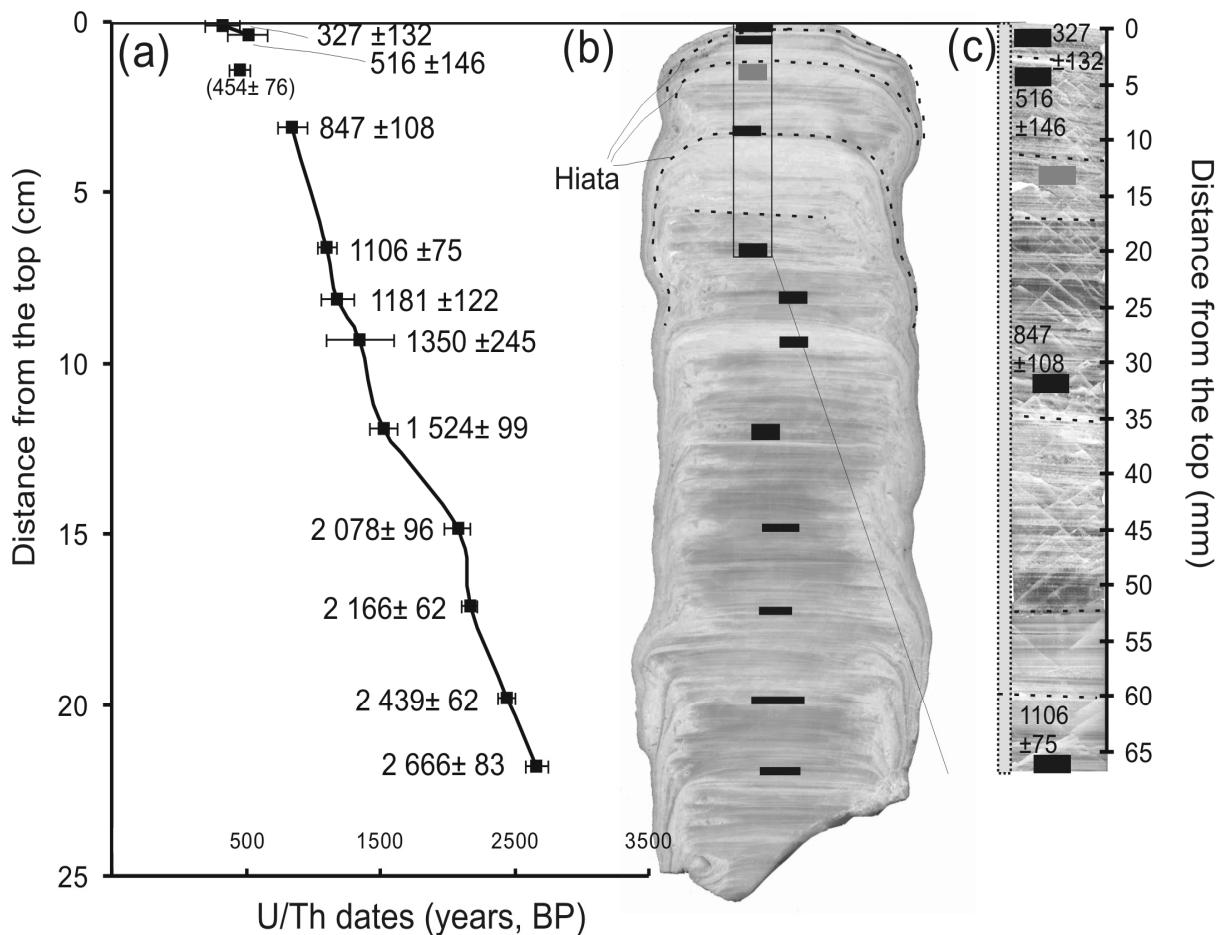
Fig. 2. The determined U-Th data series vs. the depth (a) of the studied Kisköhát Shaft stalagmite (b), and the selected part for this study (c). Vertical gray bar shows the position of the stable isotope profile (c). Position of the Multi Collector-Inductively Coupled Plasma-Mass Spectrometry (MC-ICP-MS) age data are indicated by the black regions (b and c). Dotted line represents textural changes and/or hiata during the deposition of the stalagmite. Errors of the age data are also indicated.
